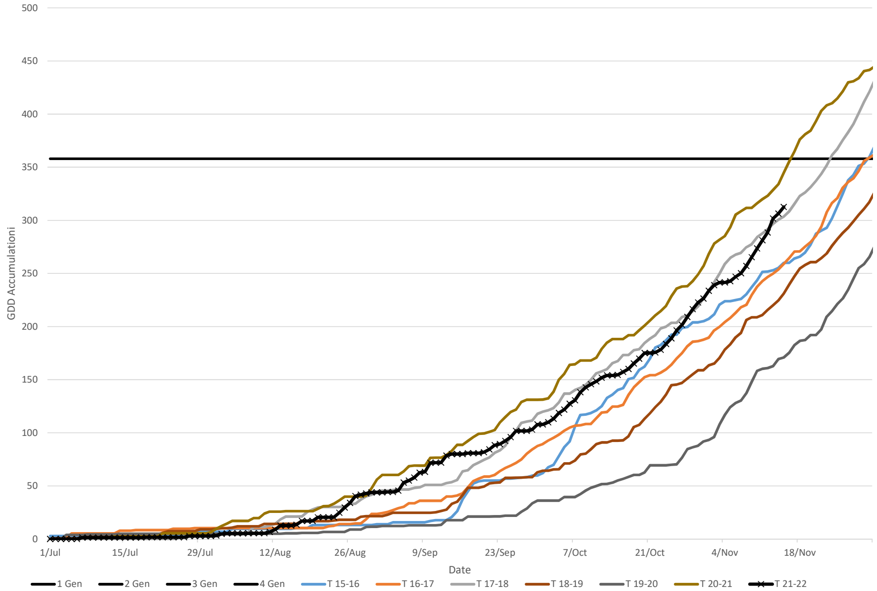
Timaru GDD Accumulation with Generations marked
