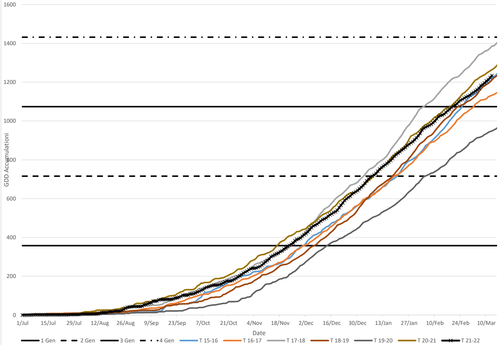
Timaru GDD Accumulation with Generations marked
