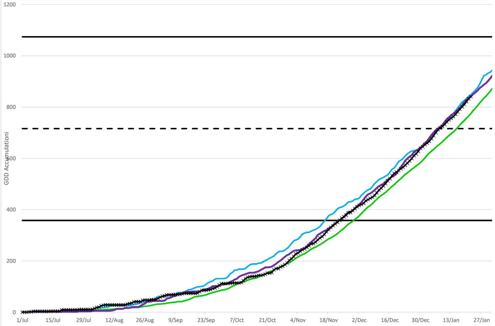
7.2 Base Timaru GDD Accumulation with Generations marked
