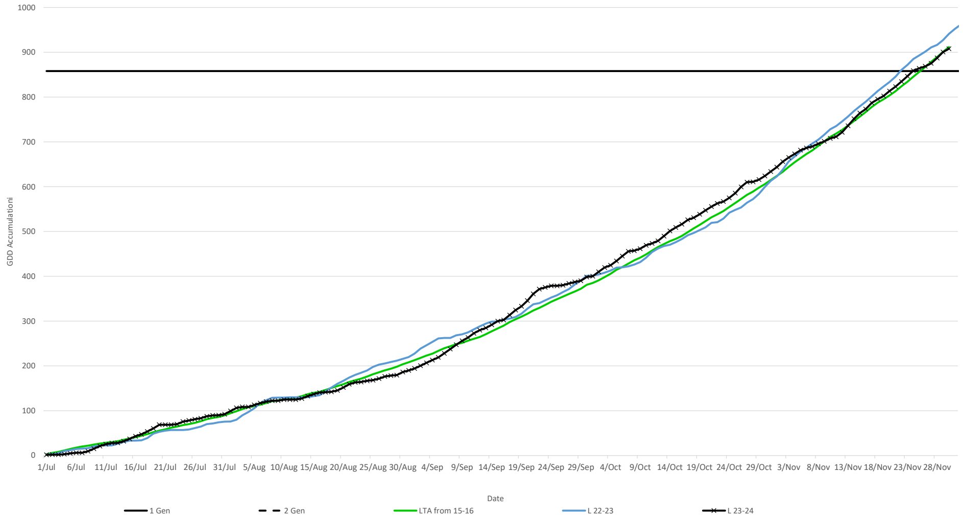
4.4 base Lincoln GDD Accumulation with Generations marked
