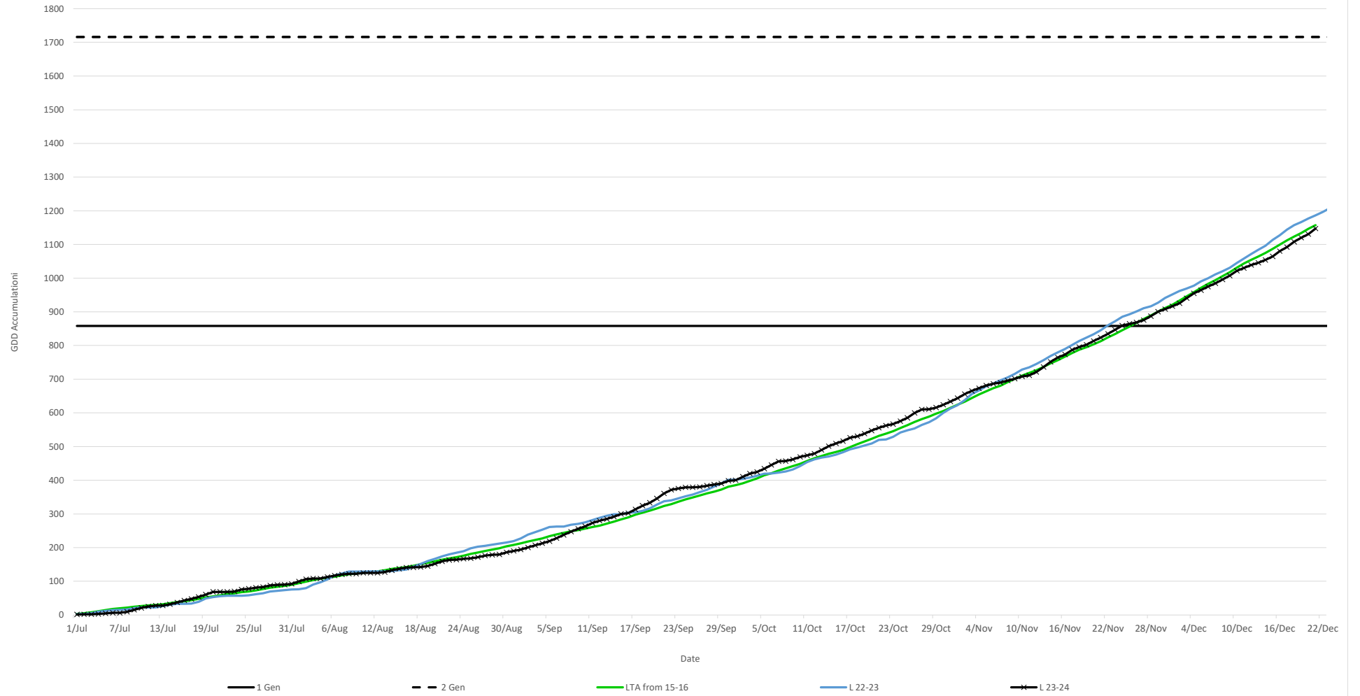
4.4 base Lincoln GDD Accumulation with Generations marked
