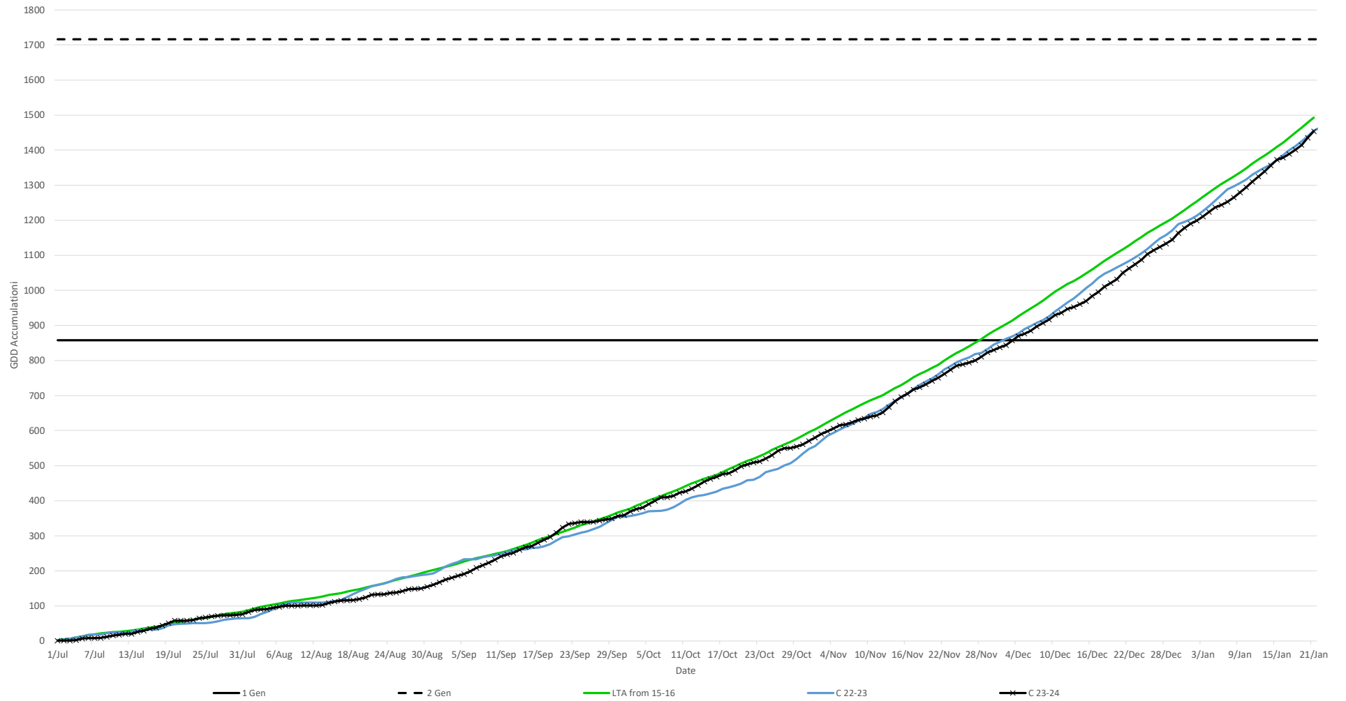
4.4 Base Chertsey GDD Accumulation with Generations marked (26-July to 11-Aug, 15-Jan-24 & 21-Jan-24, Ashburton data used due to missing data)
