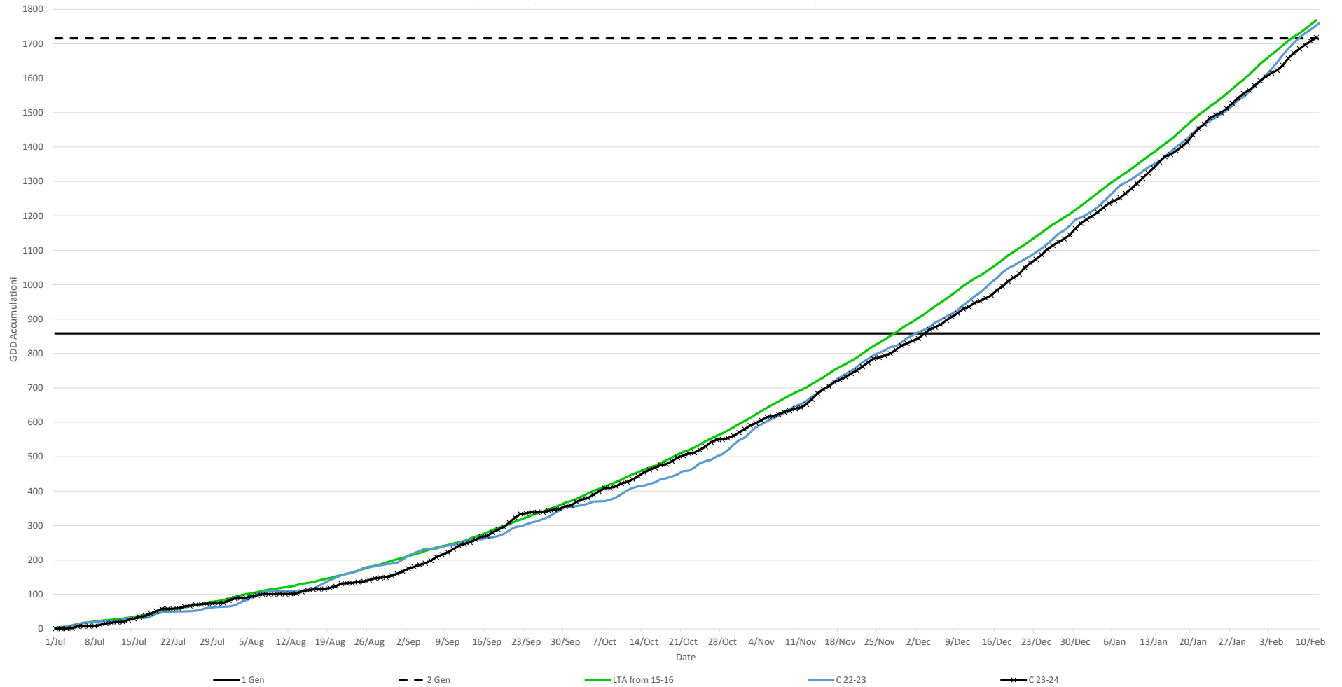
4.4 Base Chertsey GDD Accumulation with Generations marked (26-July to 11-Aug, 15-Jan-24 & 24-Jan-24, Ashburton data used due to missing data)
