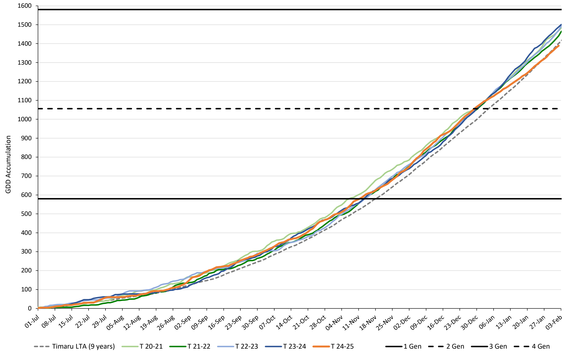
TPP GDD Accumulation at Timaru with Generations Marked (4.4°C Base)
