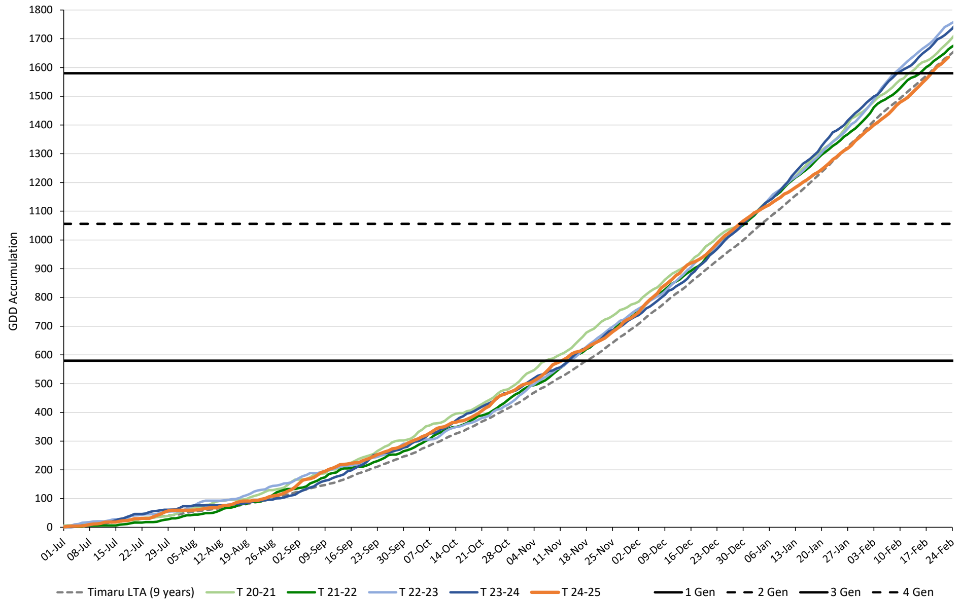
TPP GDD Accumulation at Timaru with Generations Marked (4.4°C Base)
