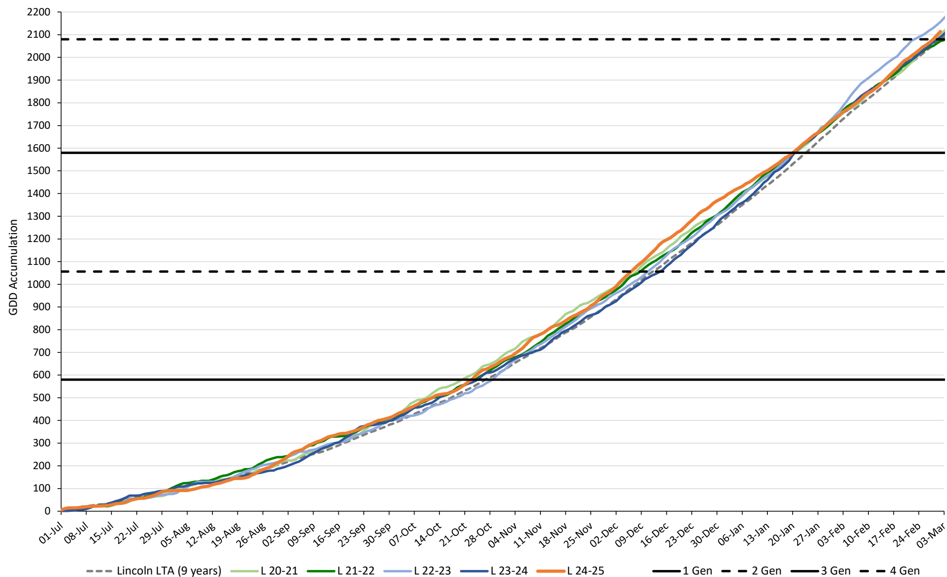
TPP GDD Accumulation at Lincoln with Generations Marked (4.4°C Base)
