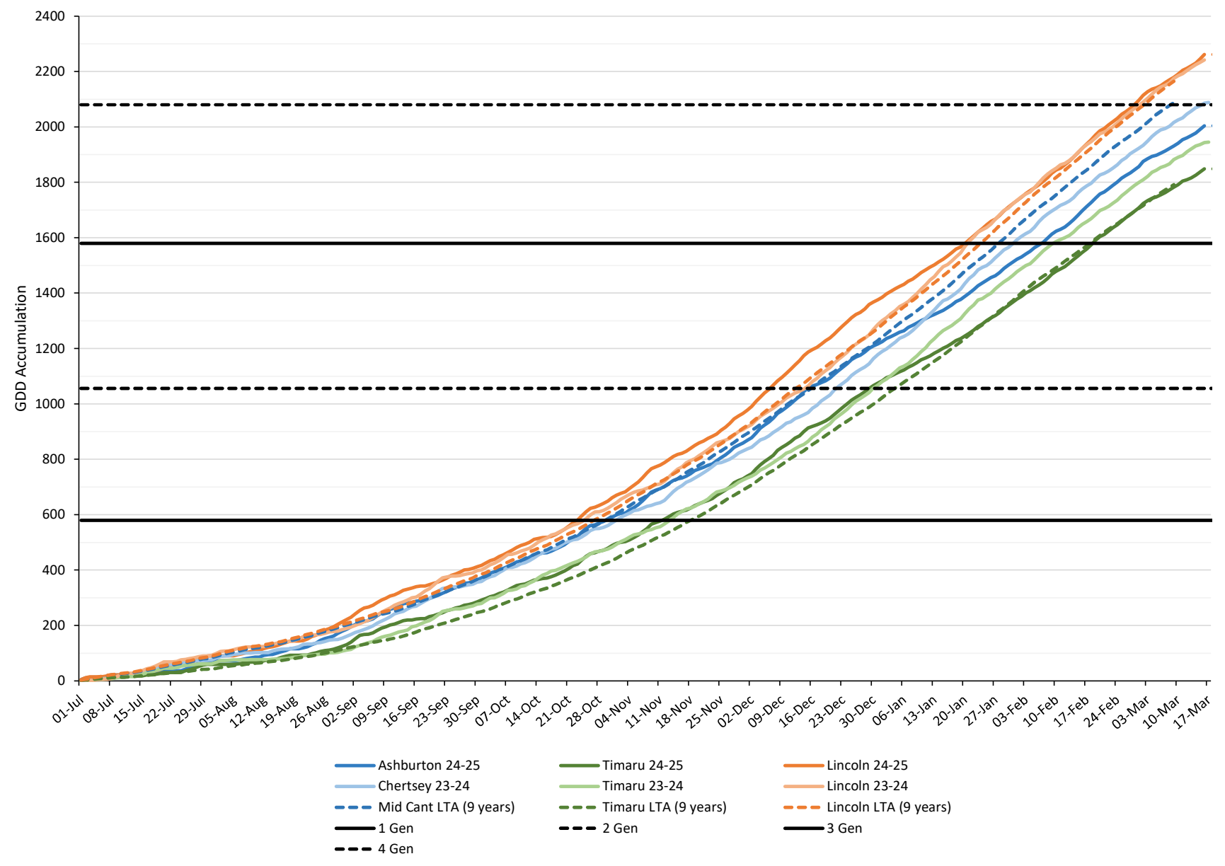
TPP GDD Accumulation at Canterbury Sites (4.4°C Base)
