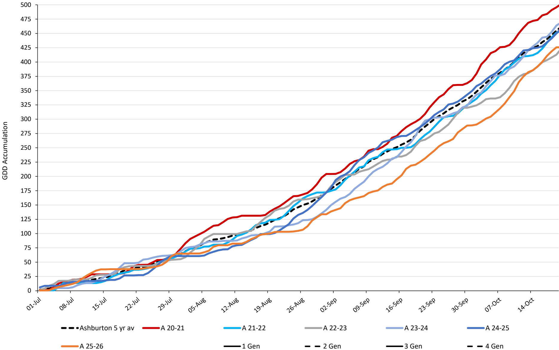
TPP GDD Accumulation in Ashburton with Generations Marked (4.4°C Base). Up to 19 October
