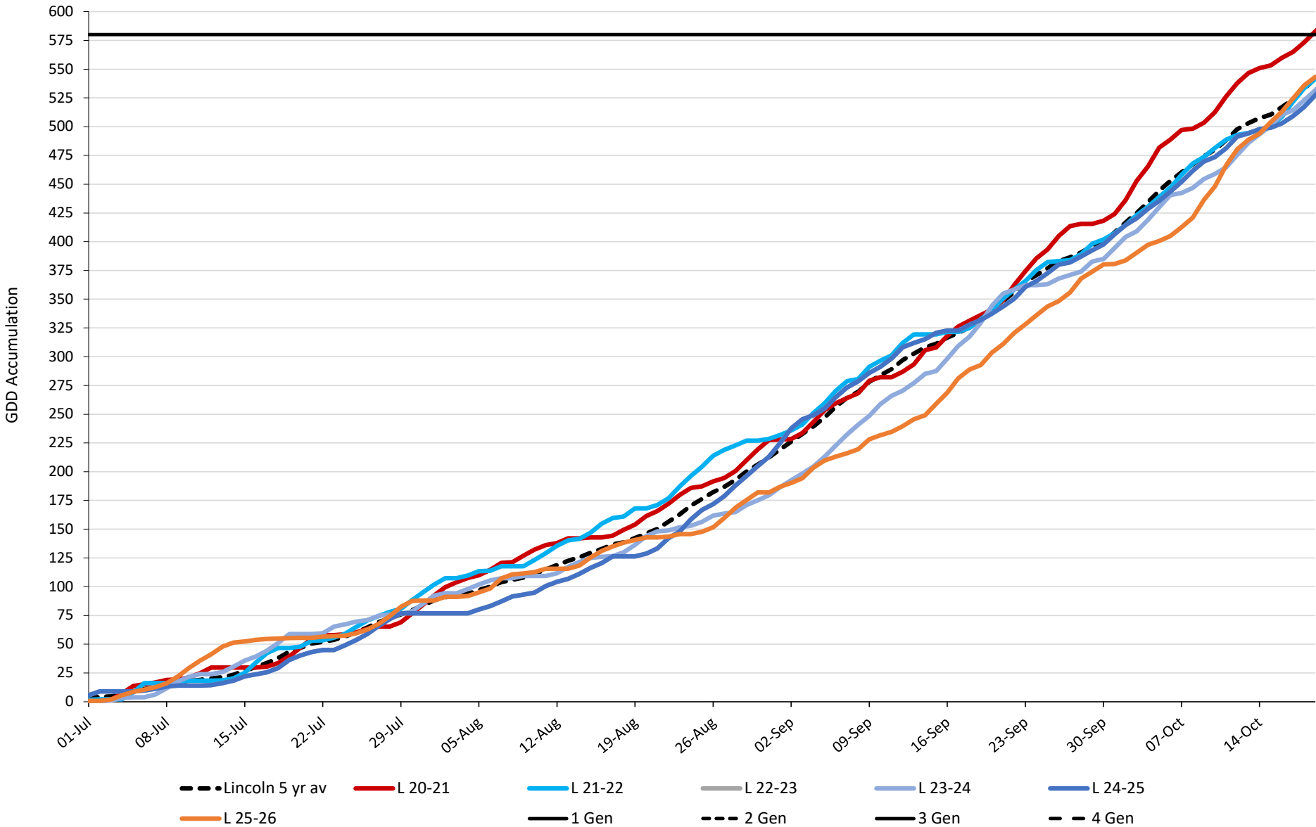
TPP GDD Accumulation at Lincoln with Generations Marked (4.4°C Base). Up to 19 October
