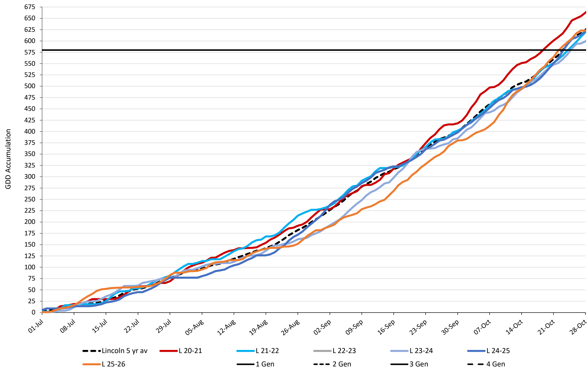
TPP GDD Accumulation at Lincoln with Generations Marked (4.4°C Base). Up to 27 October
