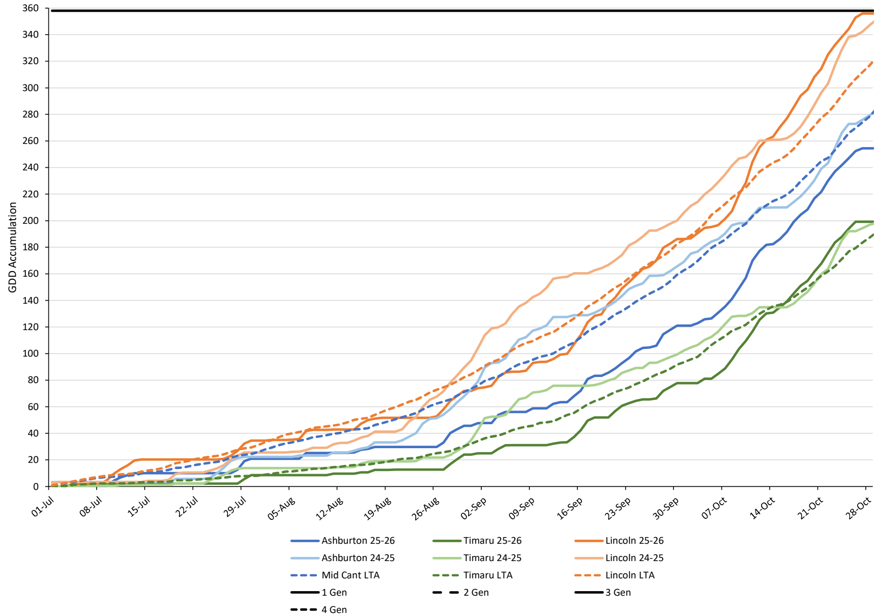
TPP GDD Accumulation (7.2°C Base) - Up to 27 October
