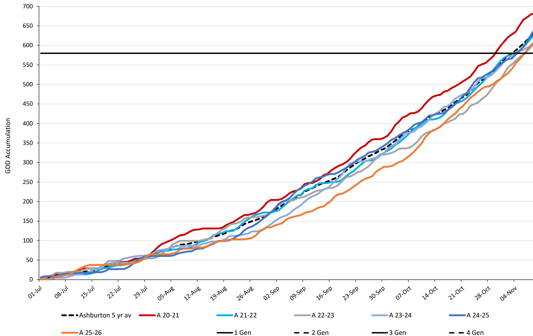
TPP GDD Accumulation in Ashburton with Generations Marked (4.4°C Base). Up to 9 November
