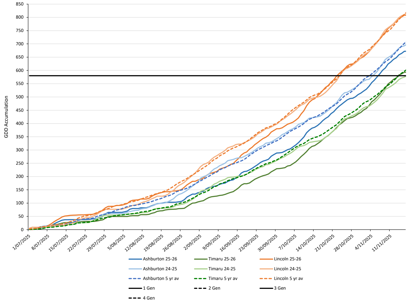
TPP GDD Accumulation at Canterbury Sites (4.4°C Base) - up to 16 November
