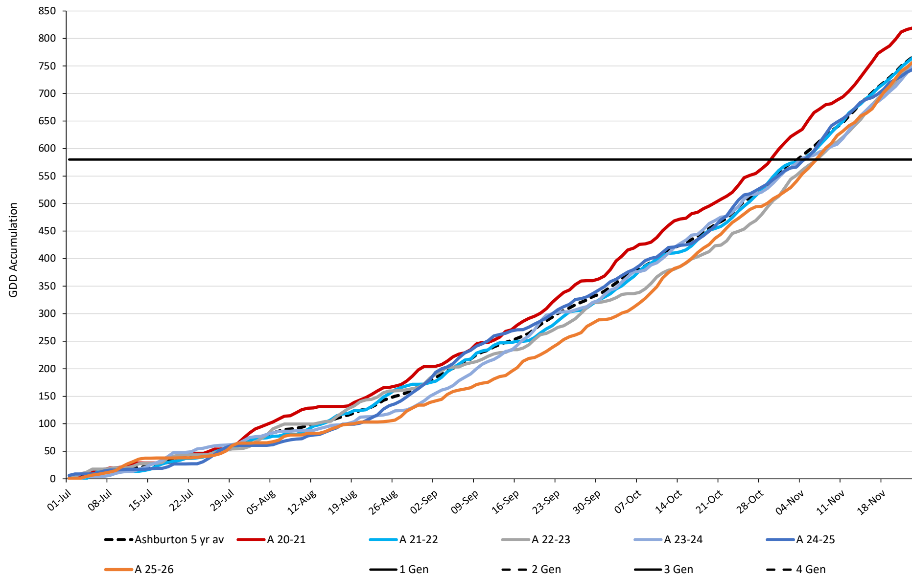
TPP GDD Accumulation in Ashburton with Generations Marked (4.4°C Base). Up to 23 November
