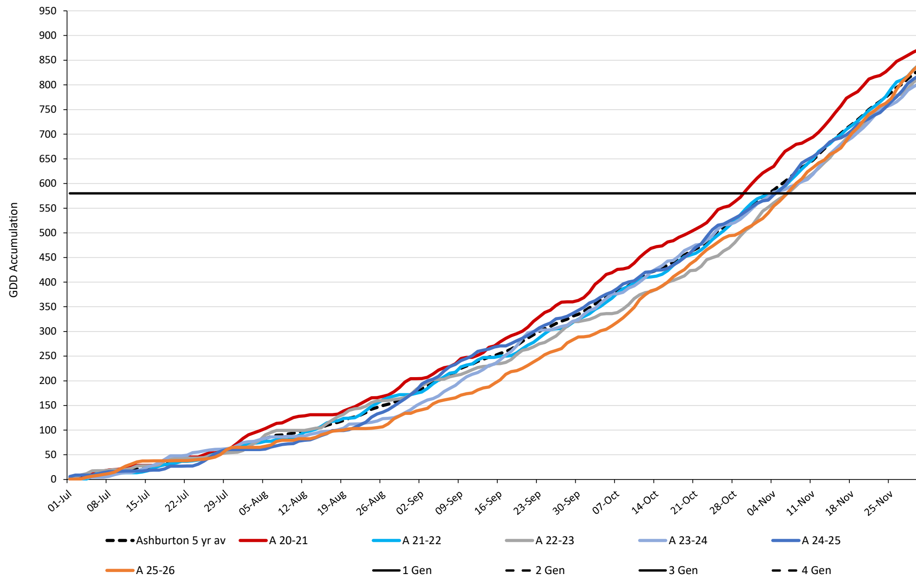
TPP GDD Accumulation in Ashburton with Generations Marked (4.4°C Base). Up to 30 November
