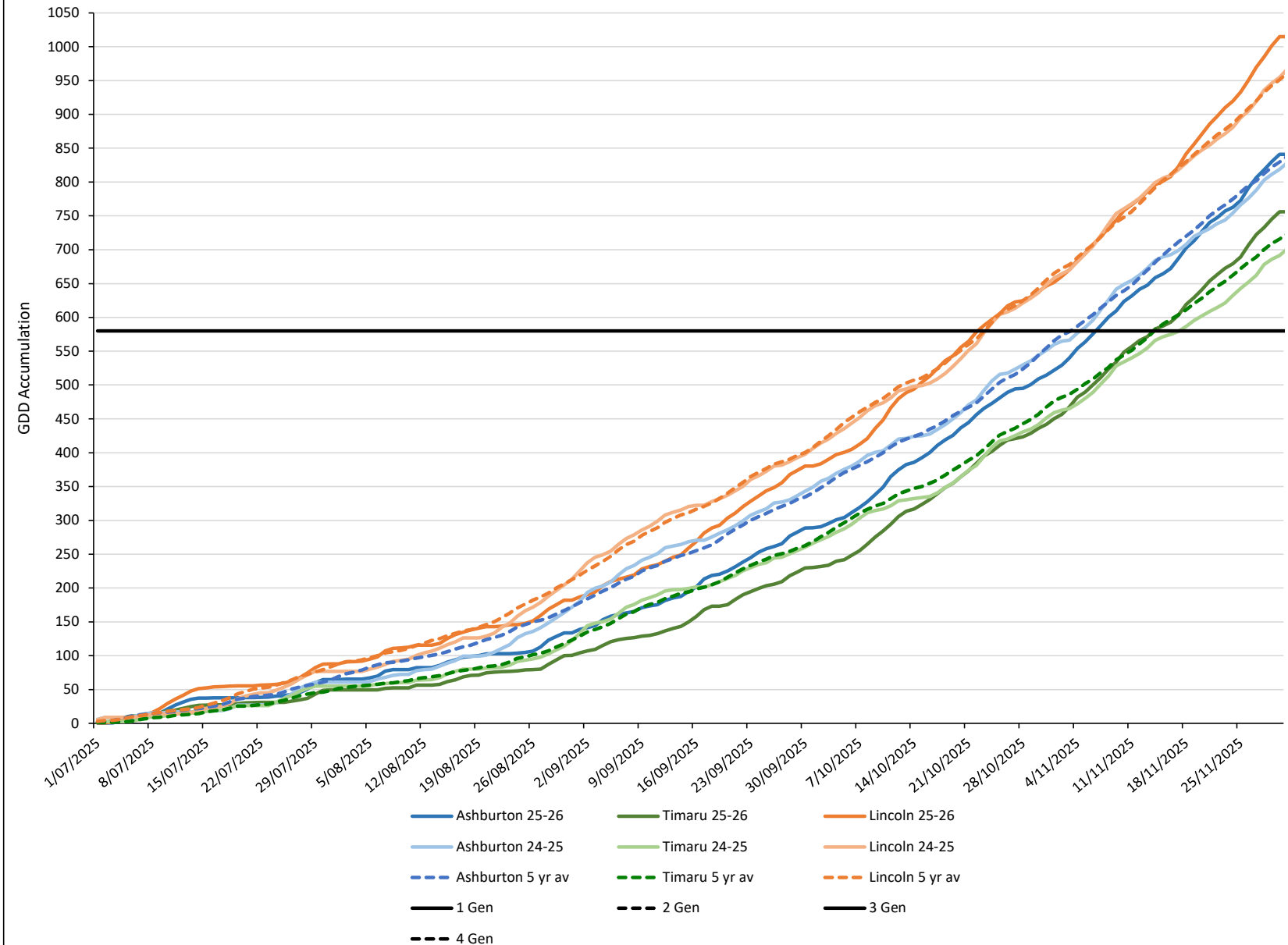
TPP GDD Accumulation at Canterbury Sites (4.4°C Base) - up to 30 November
