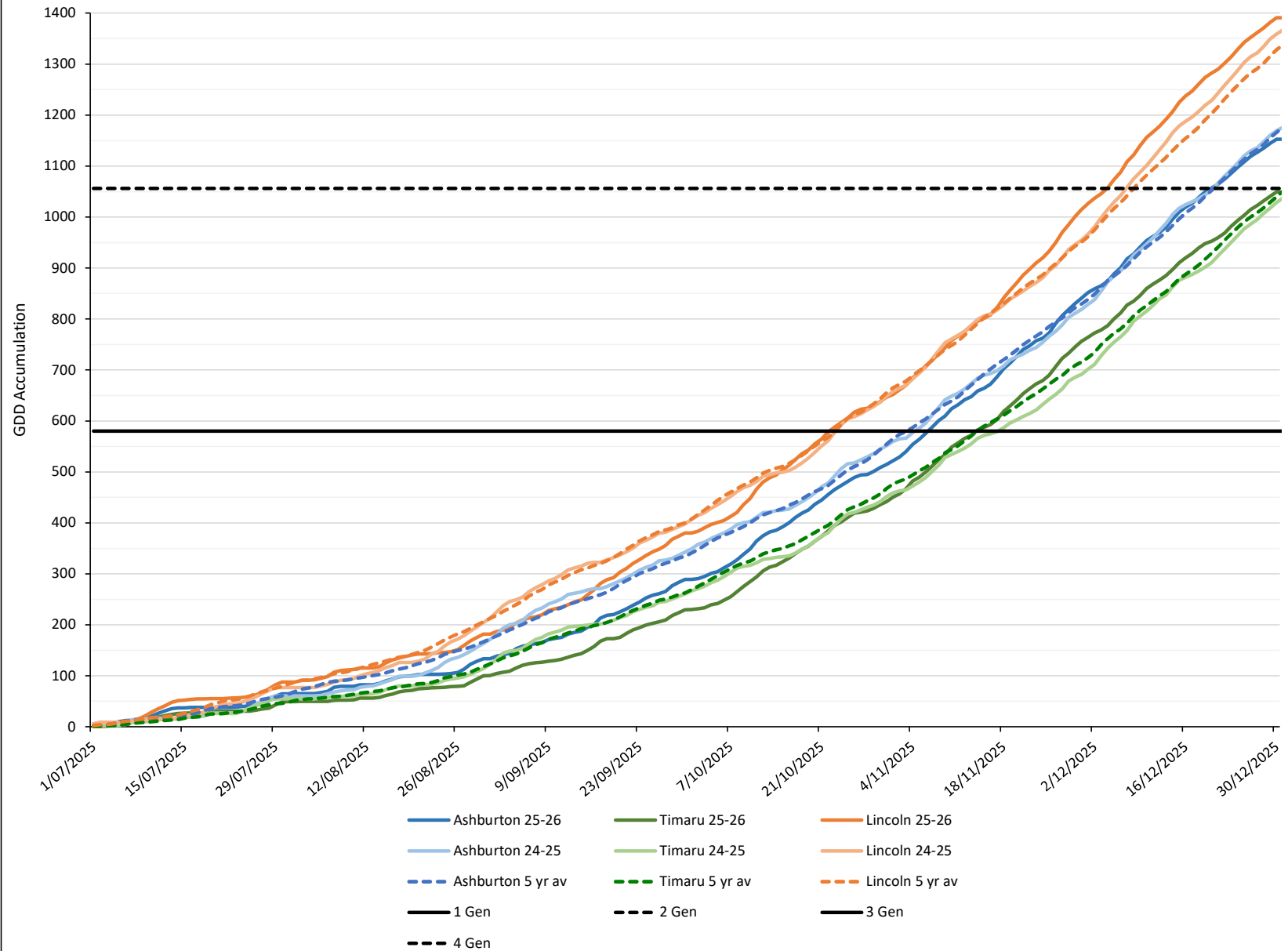
TPP GDD Accumulation at Canterbury Sites (4.4°C Base) - up to 30 December
