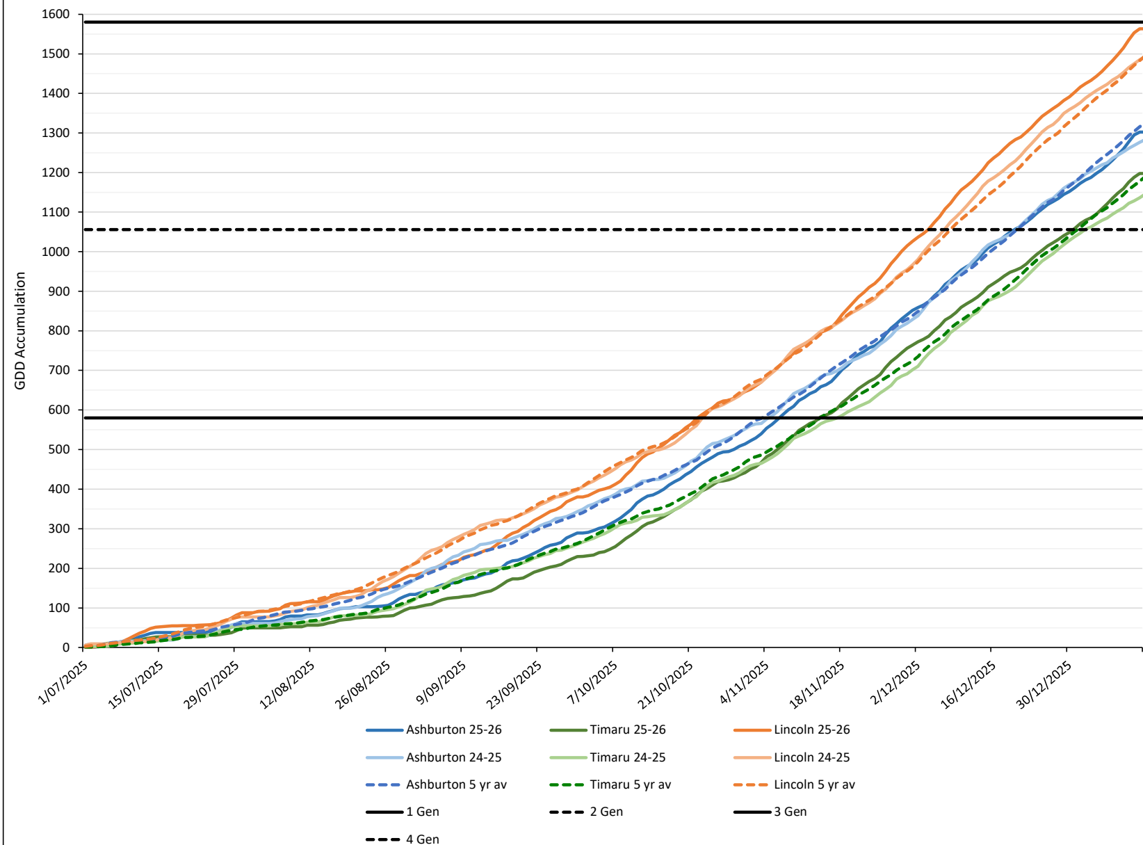
TPP GDD Accumulation at Canterbury Sites (4.4°C Base) - up to 12 January
