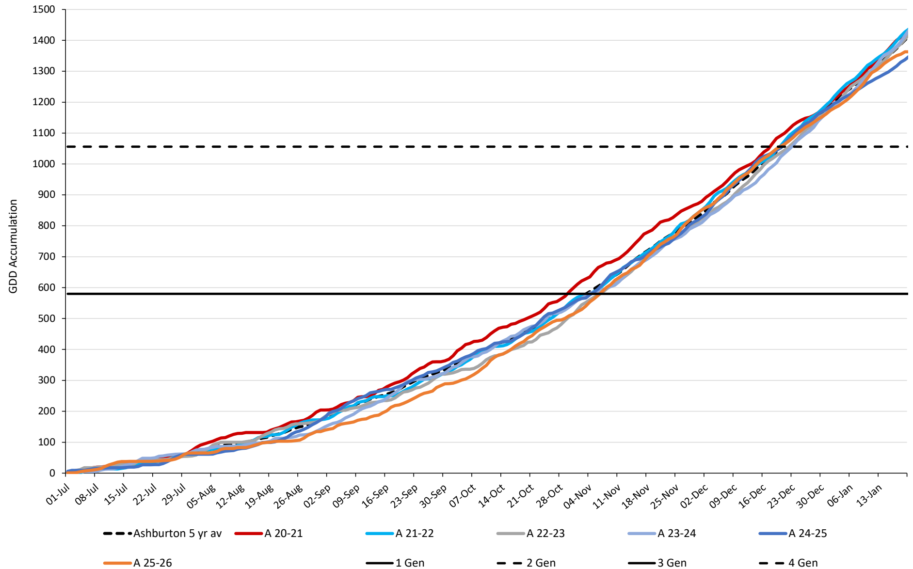
TPP GDD Accumulation in Ashburton with Generations Marked (4.4°C Base). Up to 19 January
