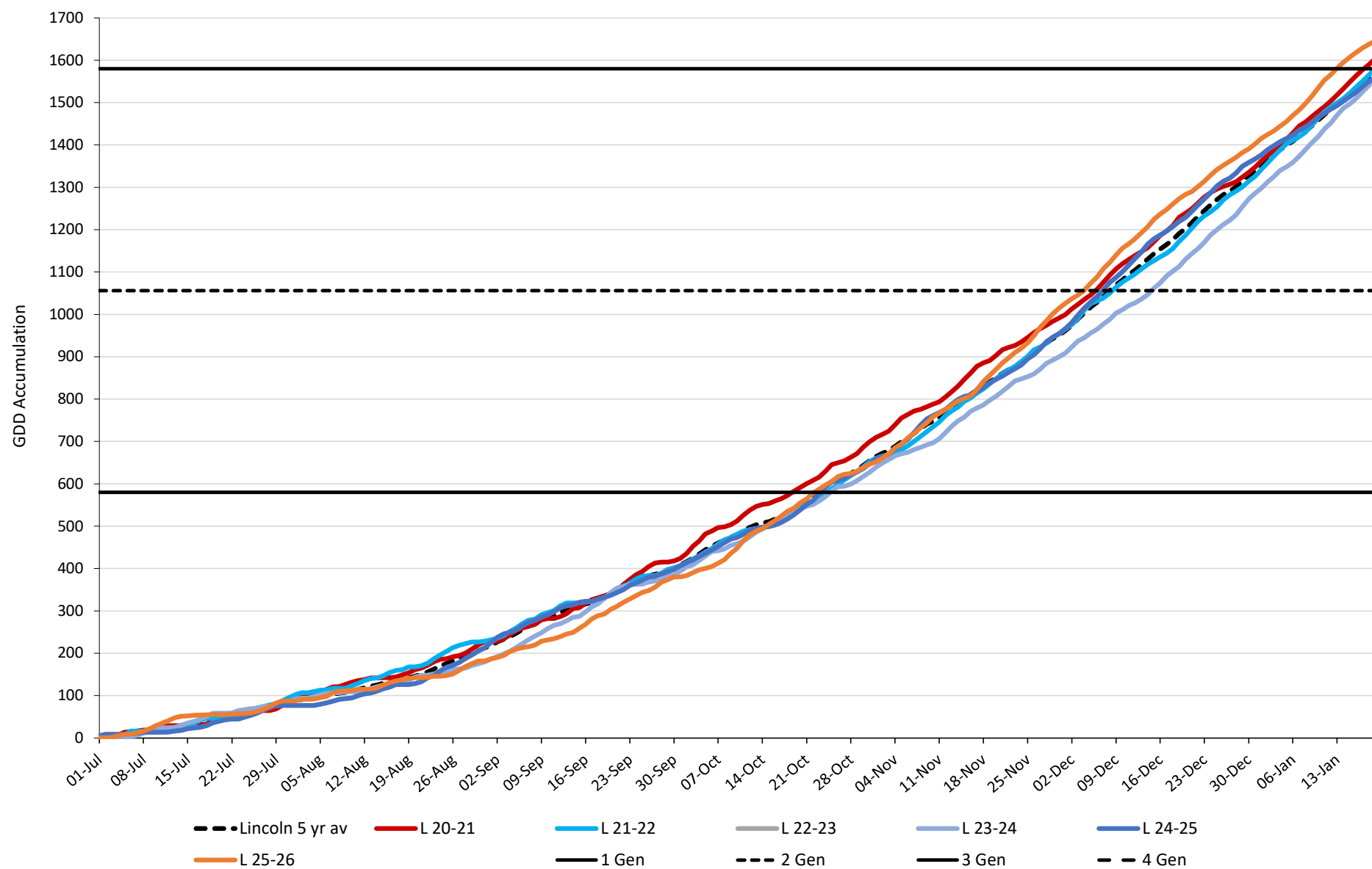
TPP GDD Accumulation at Lincoln with Generations Marked (4.4°C Base). Up to 19 January
