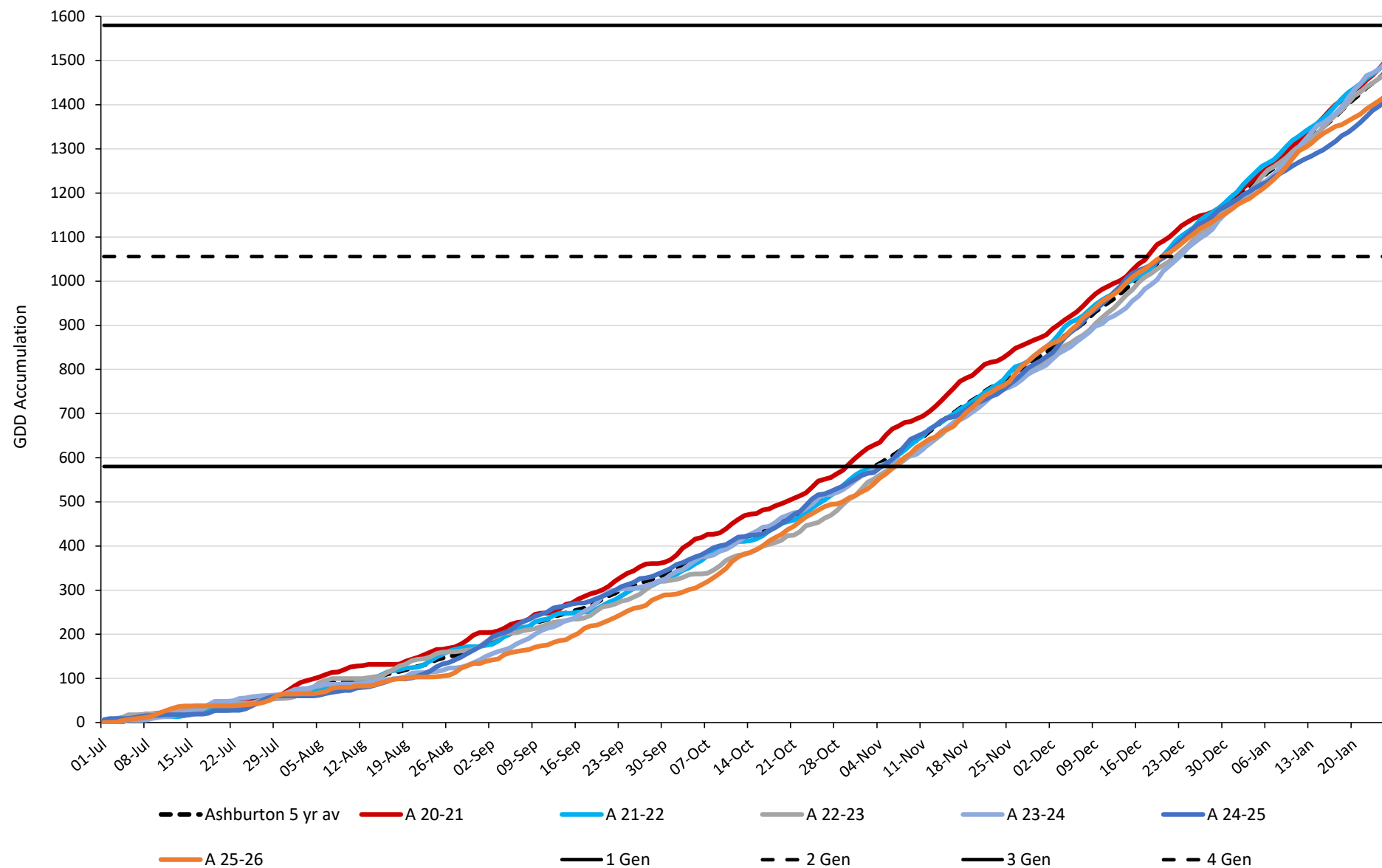
TPP GDD Accumulation in Ashburton with Generations Marked (4.4°C Base). Up to 25 January
