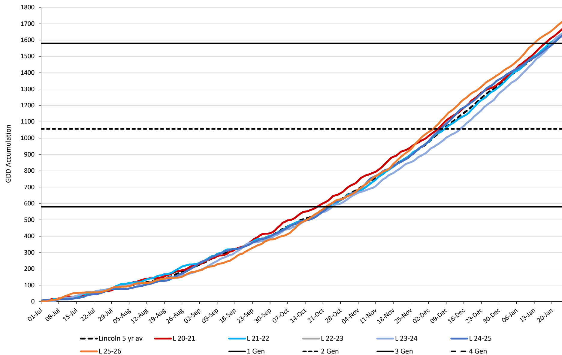
TPP GDD Accumulation at Lincoln with Generations Marked (4.4°C Base). Up to 25 January
