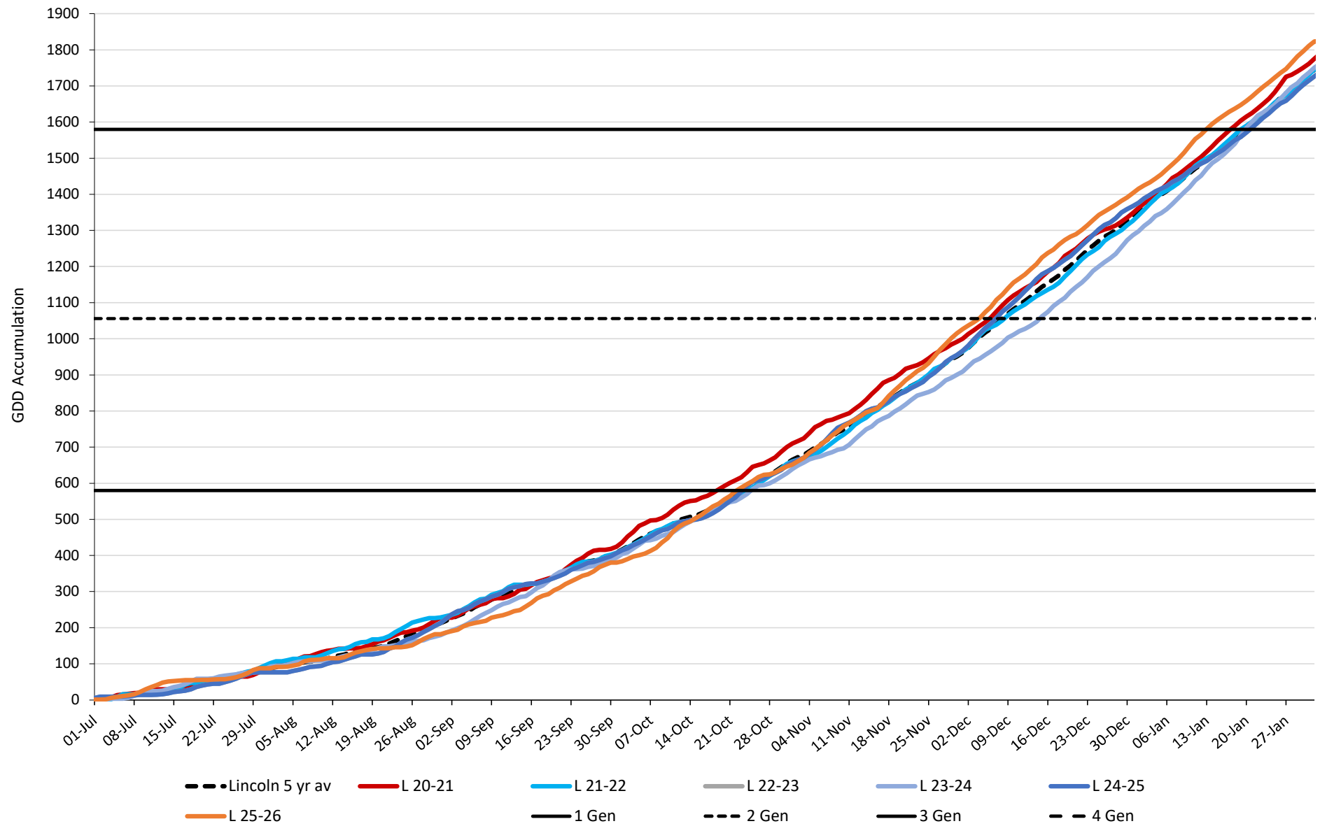
TPP GDD Accumulation at Lincoln with Generations Marked (4.4°C Base). Up to 1 February
