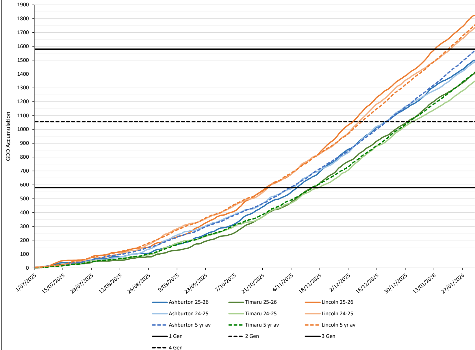
TPP GDD Accumulation at Canterbury Sites (4.4°C Base) - up to 1 February
