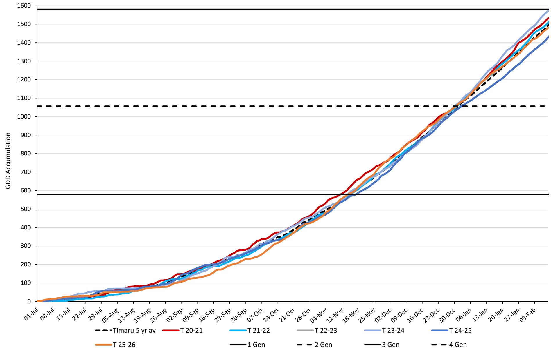
TPP GDD Accumulation at Timaru with Generations Marked (4.4°C Base). Up to 9 February
