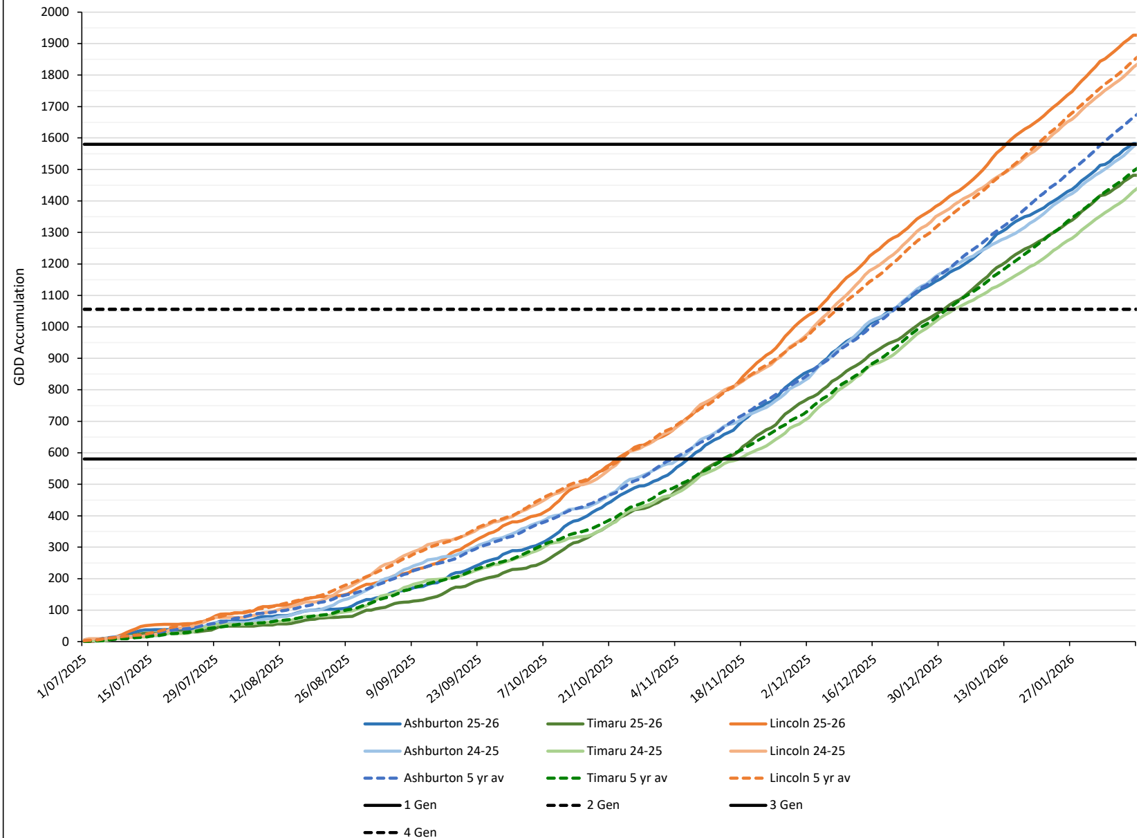
TPP GDD Accumulation at Canterbury Sites (4.4°C Base) - up to 9 February
