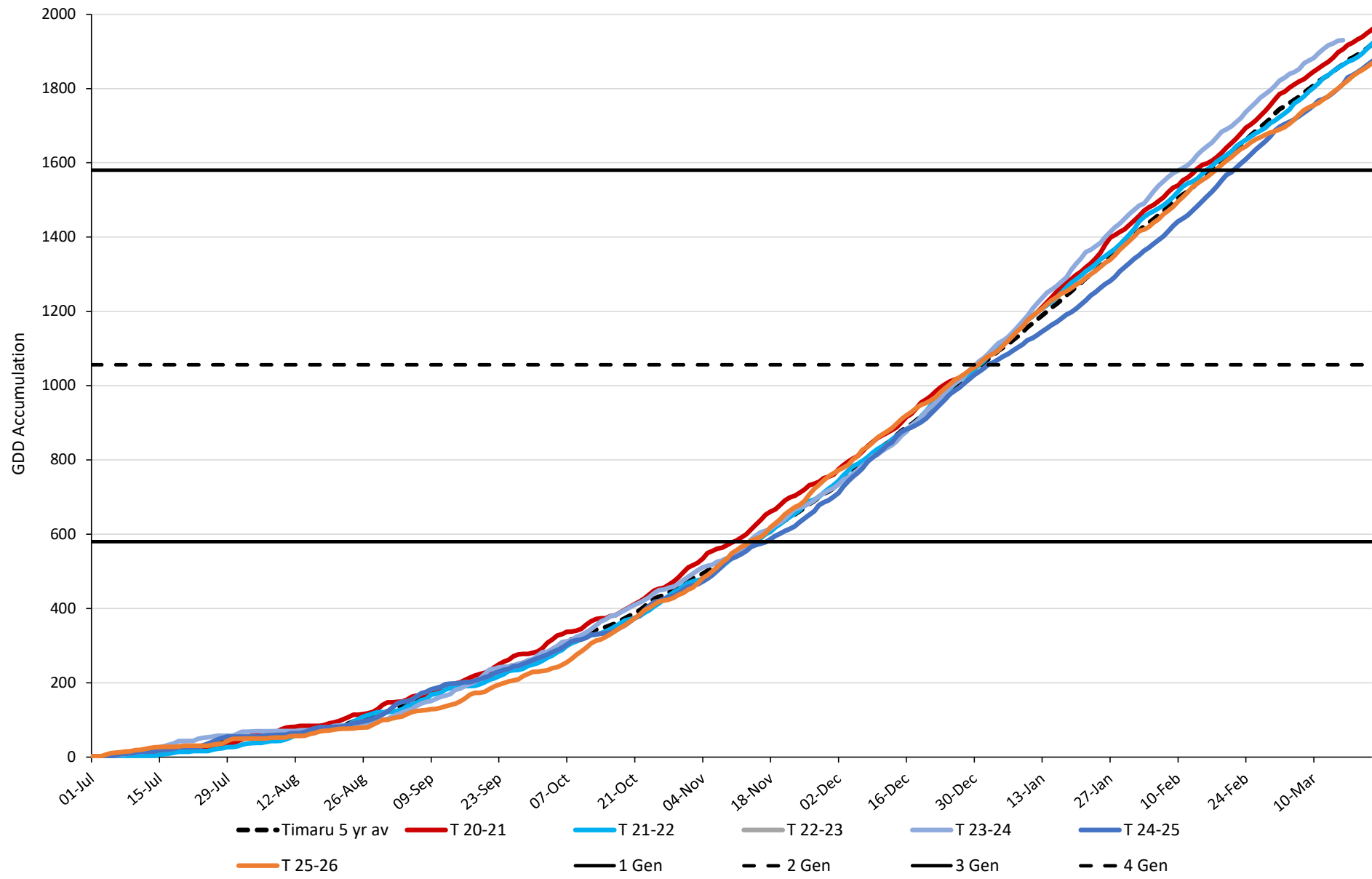
TPP GDD Accumulation at Timaru with Generations Marked (4.4°C Base). Up to 22 March
